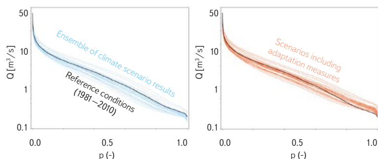
Fig. 6. Effects of climate change by 2050 on flow duration curves for mean daily discharge in the upper Svatka catchment (station 4420 – Dalečín): direct effects of climate change (left) and effects following implementation of the complex adaptation measure “hydrologically optimal agriculture” (right). The curves are based on daily modelled discharge. Individual coloured lines represent the 26 model scenarios
