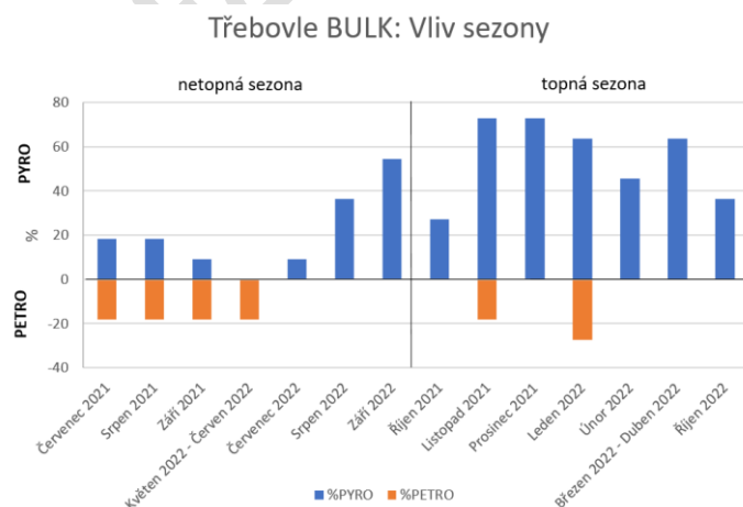
Fig. 13. Average contribution of PAHs sources in selected matrices
